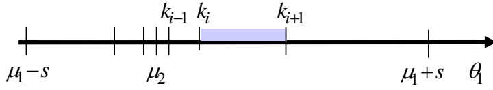
Figure 1: Communication Equilibria under Centralization.
